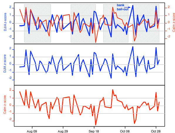
Figure 3: A panel of three graphs. The top graph shows the overlap of the day-to-day difference of DJIA values (blue: Z_{D_t} ) with the GPOMS' Calm time series (red: Z_{X_t} ) that has been lagged by 3 days. Where the two graphs overlap the Calm time series predict changes in the DJIA closing values that occur 3 days later. Areas of significant congruence are marked by gray areas. The middle and bottom graphs show the separate DJIA and GPOMS' Calm time series.
