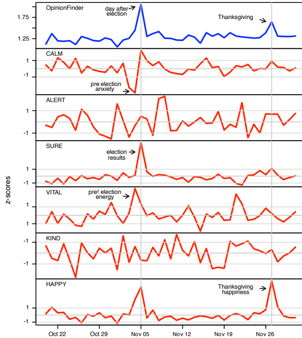
Figure 2: Tracking public mood states from tweets posted between October 2008 to December 2008 shows public responses to presidential election and thanksgiving.
